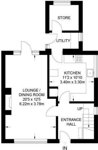
GROUND FLOOR 539 SQ FT / 50.1 SQ M
